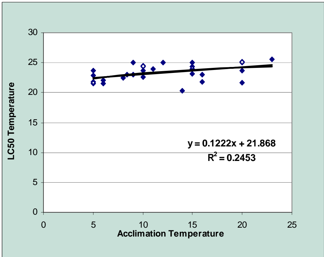
Figure 3. Combined lethality data for all salmonid species (based on 7-d LT50 constant temperature exposure test results).
